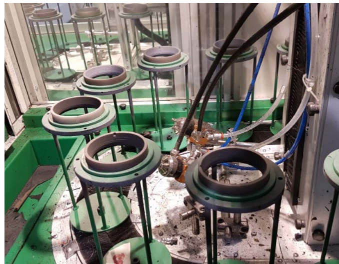
Inside coating cabin with atomization gun PA-210xx.
