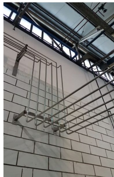
Centralized supply and recirculation line - calibrated tubes AISI 316SS
